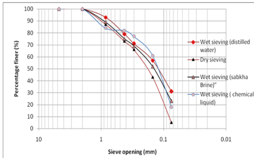
Fig. 4: Sabkha soil's grain size distribution of study samples.
