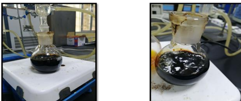
Fig. 6: The creation of stable compounds with metal ions using the novel Schiff's base of furfural (M).
